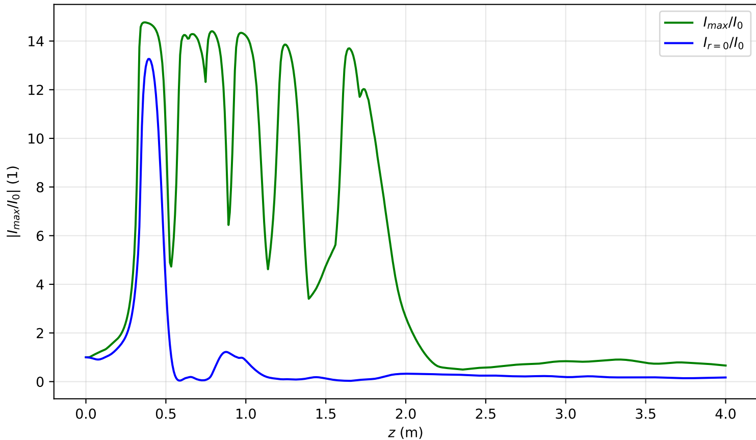
I_{max}(x=0, y=0, z)/I_0 , P_{in}=7.5P_{cr} , noisy input, artificial time
